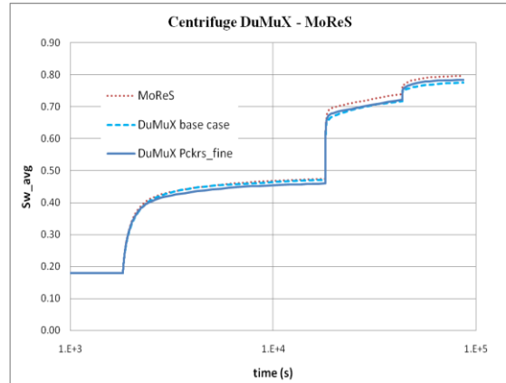
Fig. 2 Validation of DuMu x simulations against MoReS for the centrifuge demo data set. Effect of densely spaced table interpolation.
