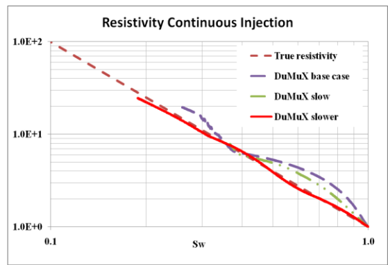
Fig. 6 Continuous Injection. Synthetic case, rate dependency resistivity measurement.
